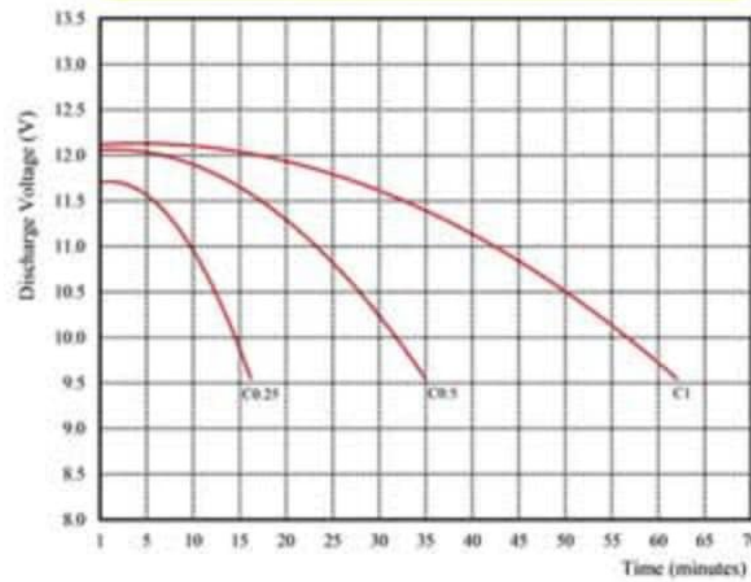
Discharging Characteristic (25°C)
