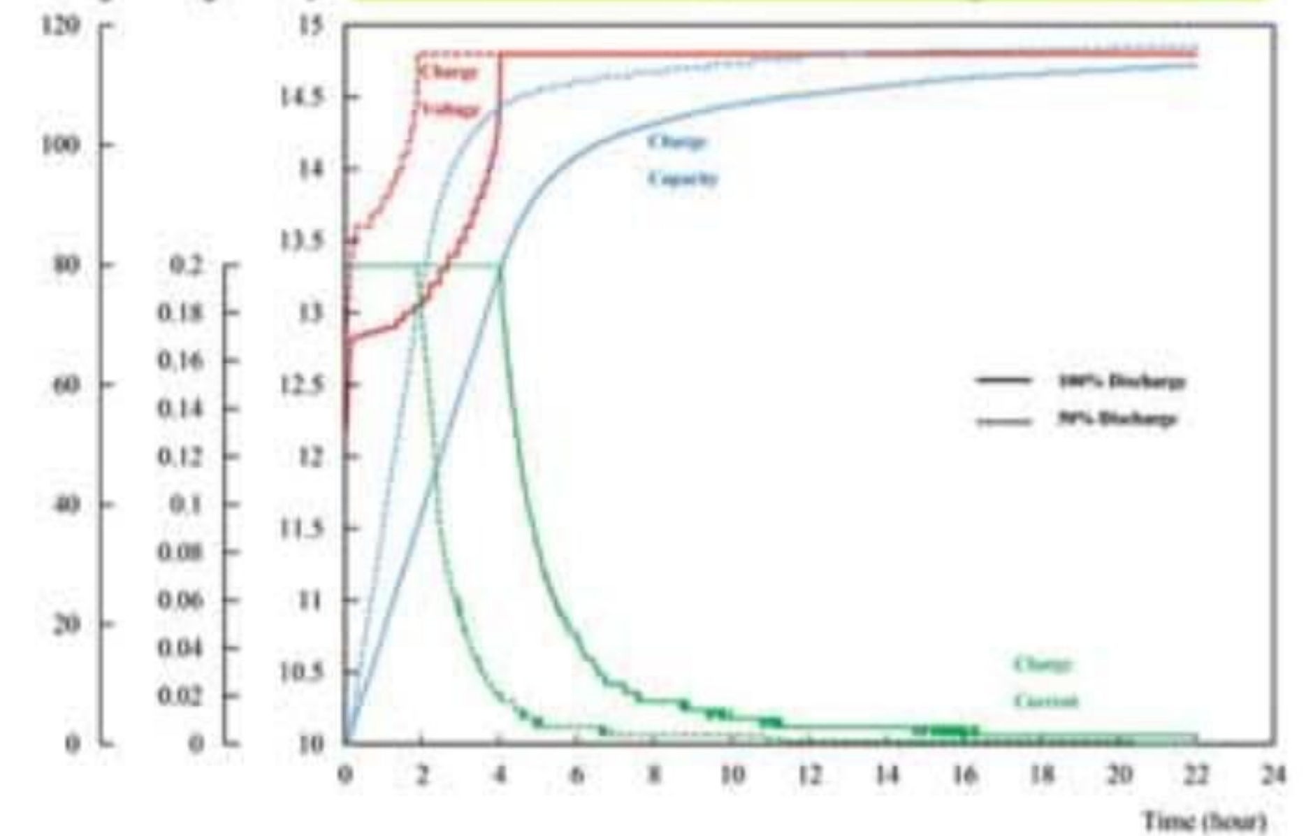
Constant Charge at 0.2CA-14.8V(25°C)
