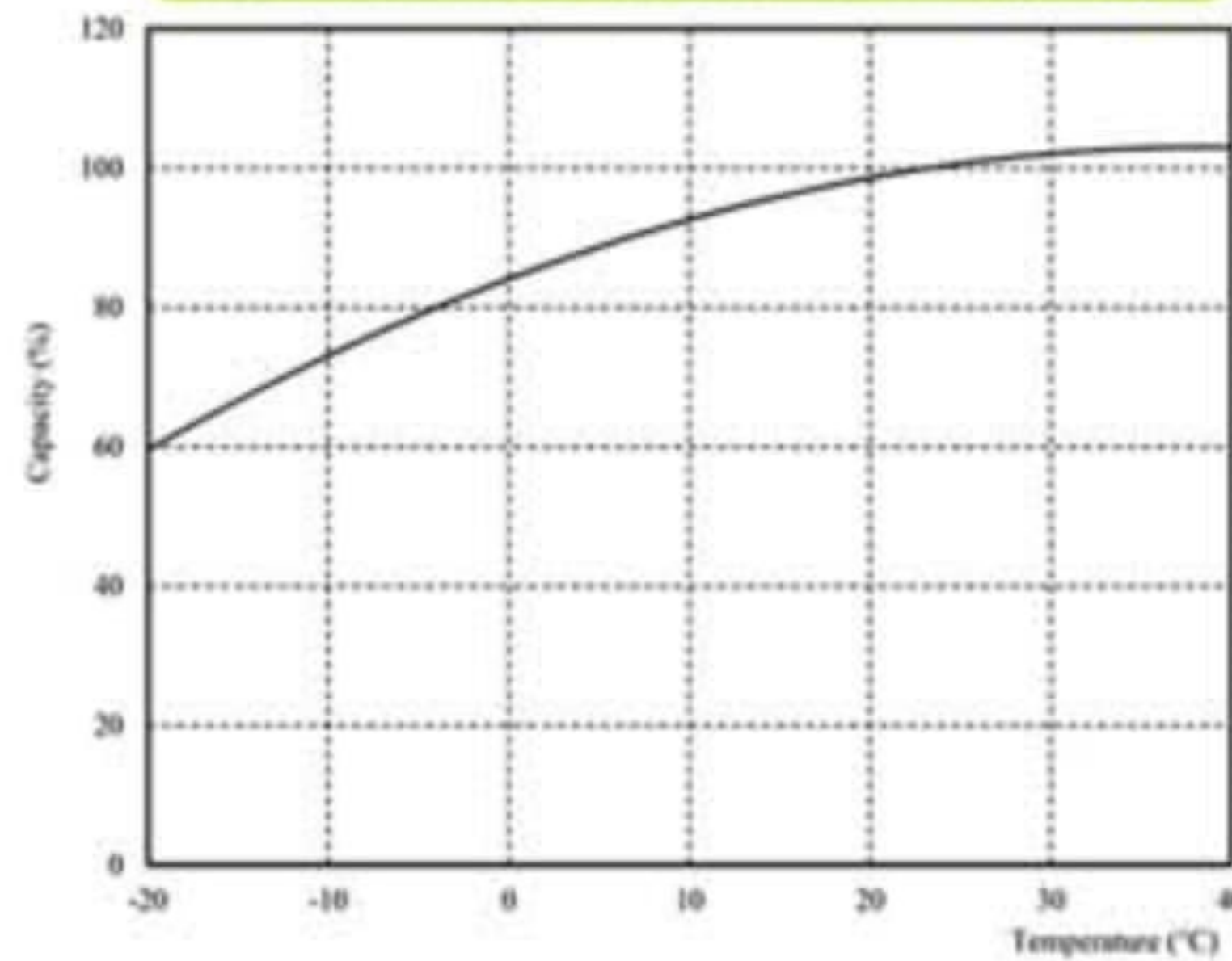
The Effect of Temperature on Capacity
