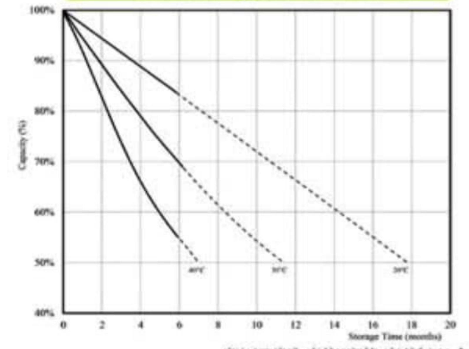
Self-Discharge Characteristics
