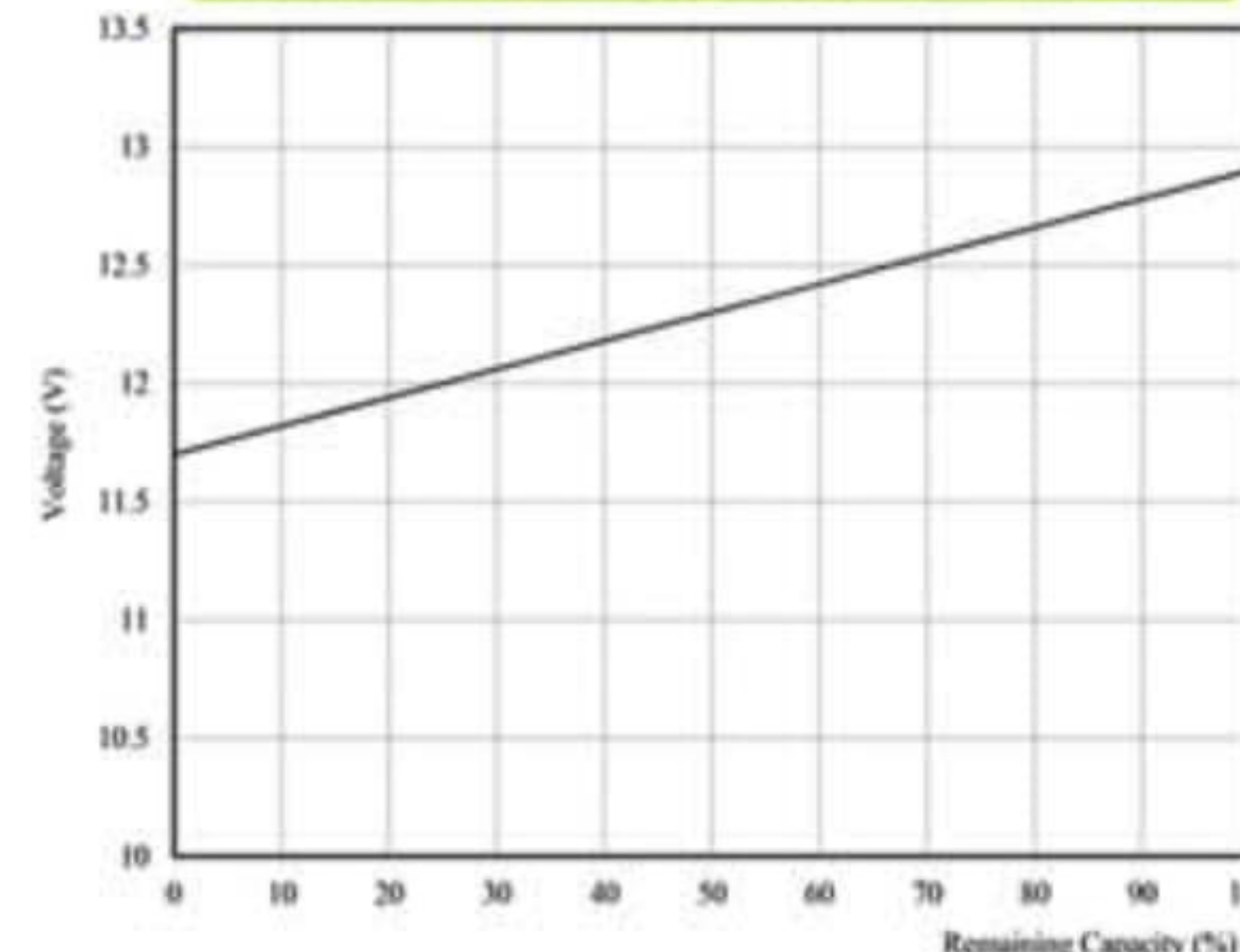
Relationship If OCV and state of charge
